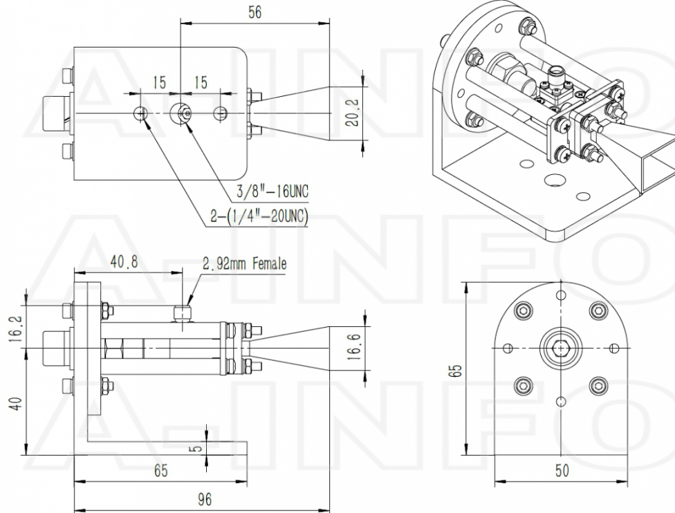
2.92mm-Female Output with L Type Mounting Bracket (Option, P/N: LB-28-10-C-MBL)
