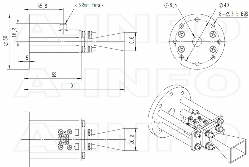
2.92mm-Female Output with Round Mounting Bracket (Option, P/N: LB-28-10-C-MB)
